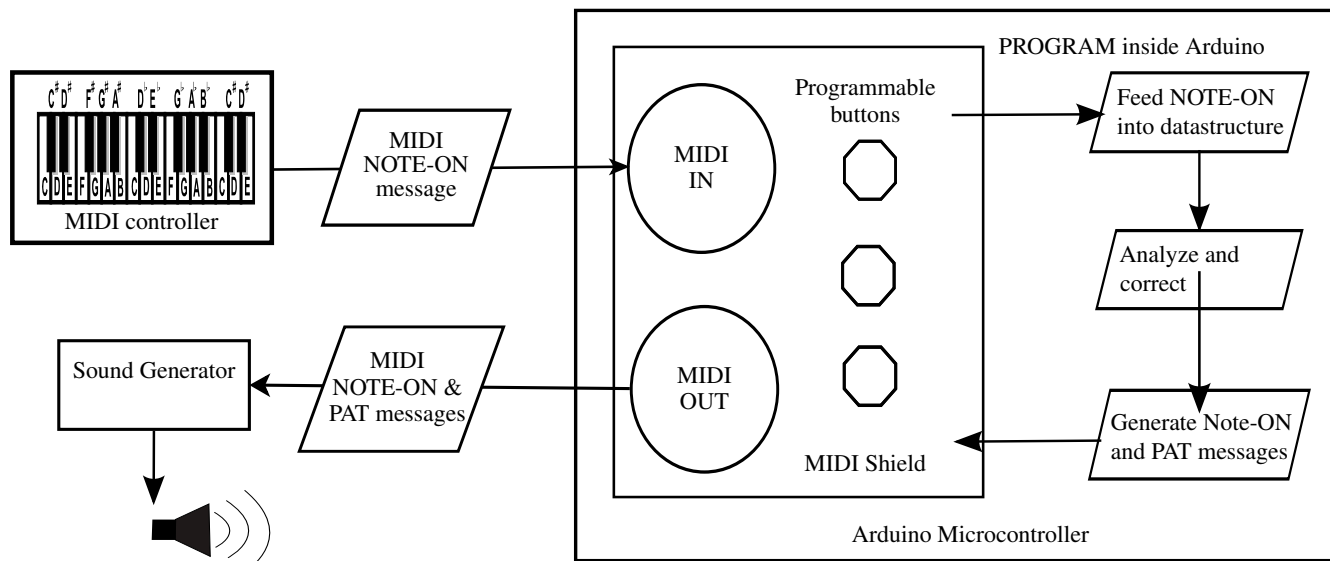
Fig. 4. Workflow of dynamic tuning.
